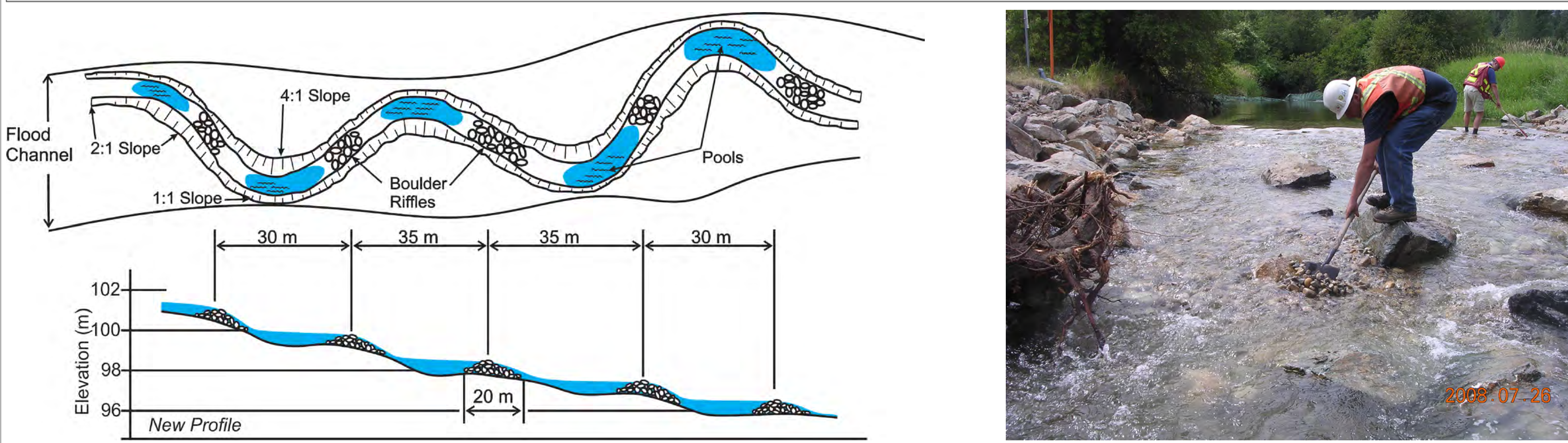
Step and Riffle Pool Construction
